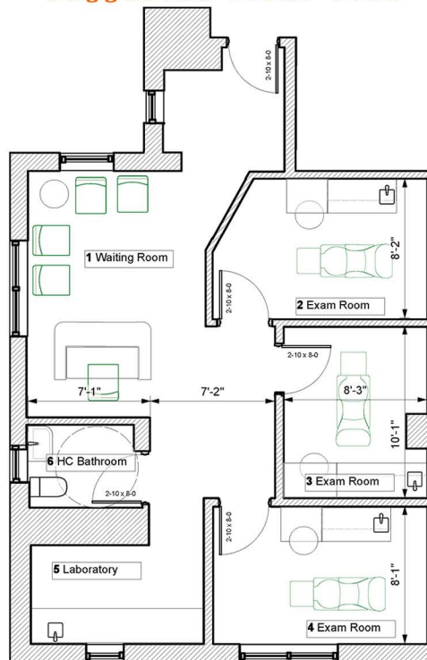
Suggested Floor Plan
